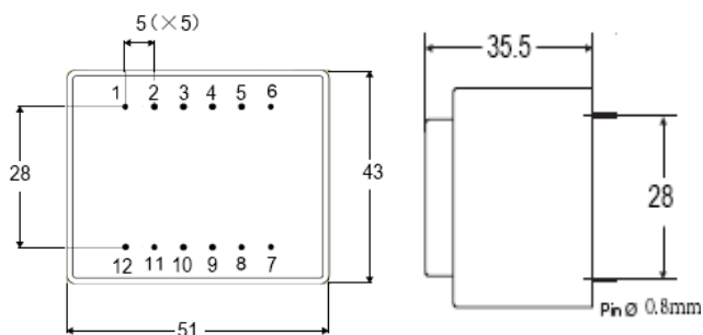
Dimension (mm)
