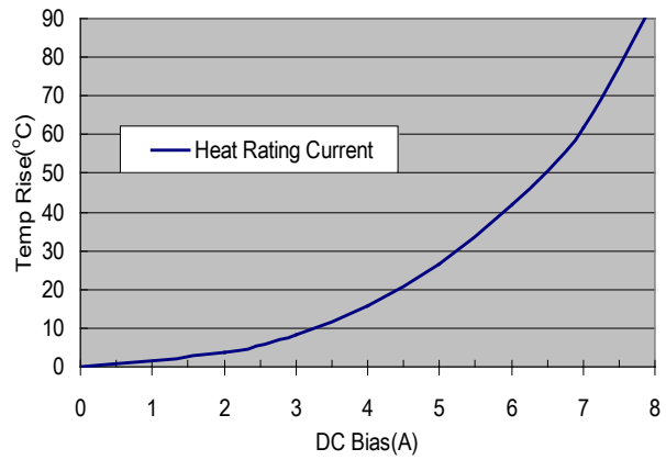
ASPI-0520LR-3R3
