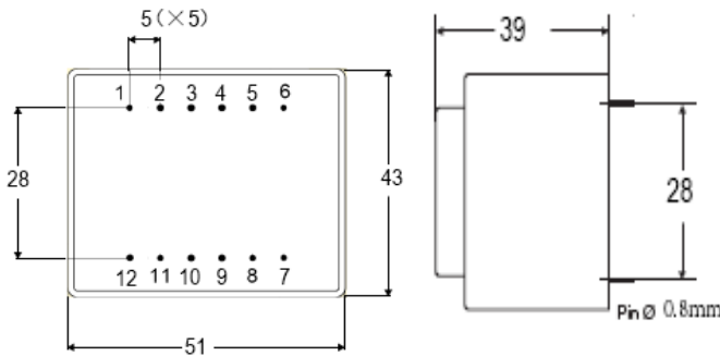
Dimension (mm)
