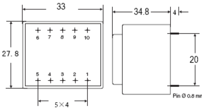
Dimension (mm)
